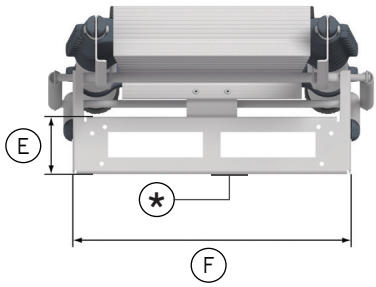
Dimension monteringsram
