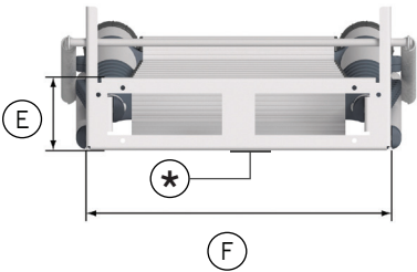
Dimension monteringsram
